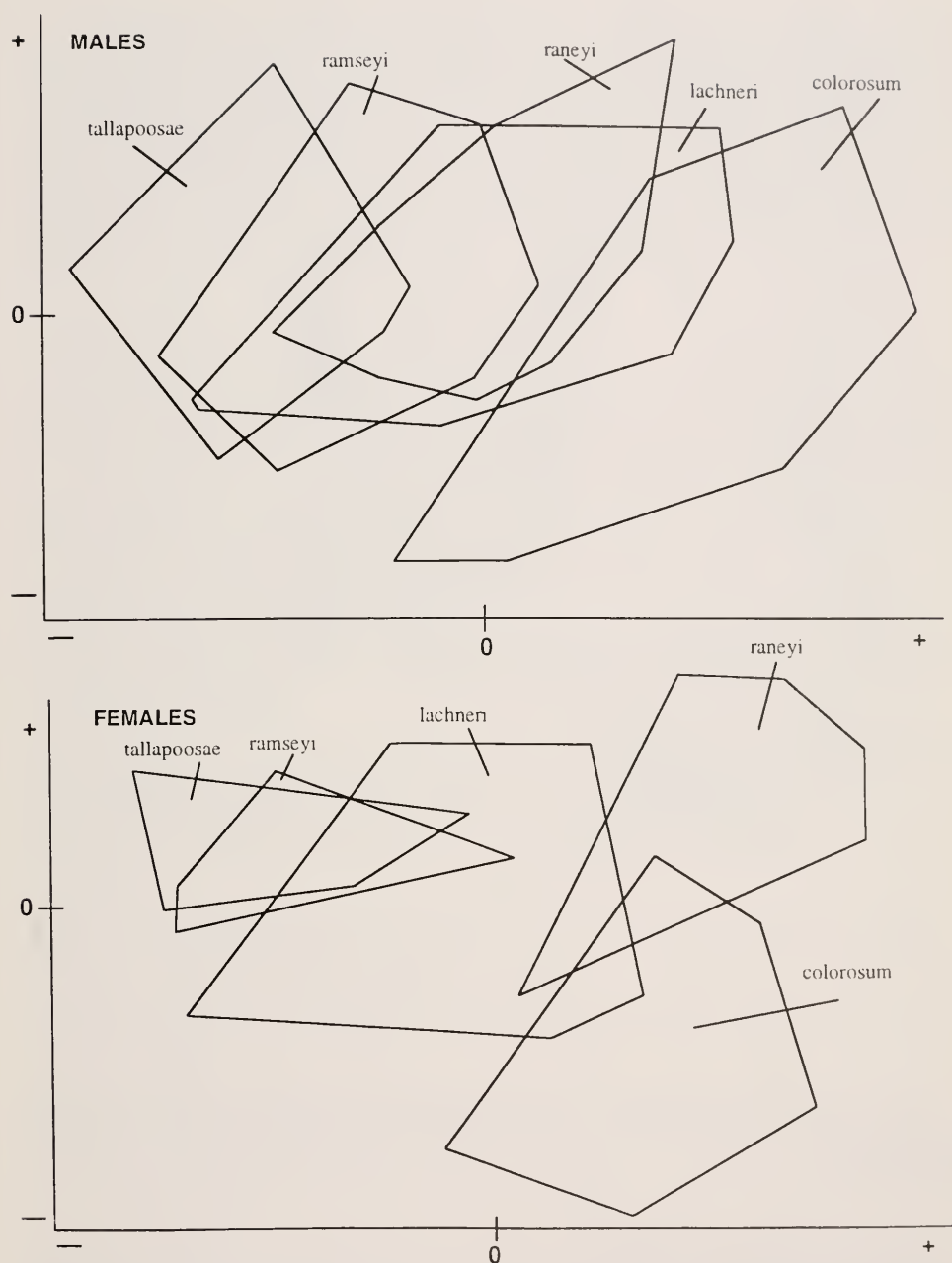
Figure 8. PCA polygons representing projections of morphometric data for Etheostoma raneyi , E. lachneri , E. ramseyi , E. tallapoosae , and E. colorosum .
