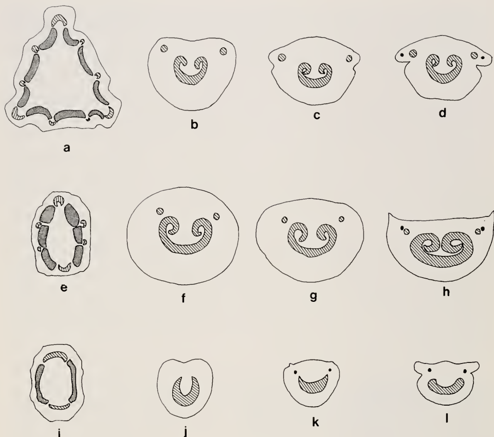
Figure 4. Selected nodal and petiolar vascular patterns from representative species of Antirhea . a—d. A. borbonica var. borbonica (St. John 26499 ♀). a. Cross section of node with whorled leaves showing for each leaf 3 traces from 3 gaps. b—d. Successive sections of petiole from base, mid-portion and distal end, showing curved vascular arc and lateral rib traces. e—h. A. megacarpa (NGF 1235 ♀) e. Cross section of node with opposite leaves showing for each leaf 3 traces from 3 gaps. f—h. Successive sections of petiole from base. i—l. A. chinensis (Lau 3150 ♂) i. Cross section of node with opposite leaves showing for each leaf 1 trace from 1 gap. j—l. Successive sections of petiole from base, mid portion and distal end respectively, showing curved vascular arc and rib traces developed at midpoint of petiole. Cross-hatched area = disrupted vascular cylinder; slashed area = leaf trace; solid area = lateral rib trace.
