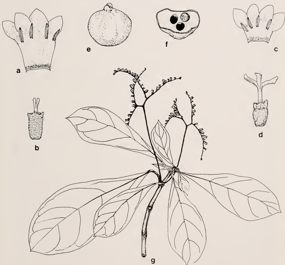
Figure 10. a—f, Antirhea bifurcata (a—b from Sieber maurit. exc. 2. n. 59. ♂; c—d from Sieber maurit. II. 199 ♀; e—f from Blackburn s.n. ♀). a—b. ♂ flower, \times 5 . c—d. ♀ flower, \times 5 . e. Fruit, \times 5 . f. Cross section of fruit, \times 5 . g. A. borbonica var. duplidivisa (27778-SF ( Capuron ) ♀), habit showing twice dichotomous inflorescence (after anthesis), \times 0.5 .
