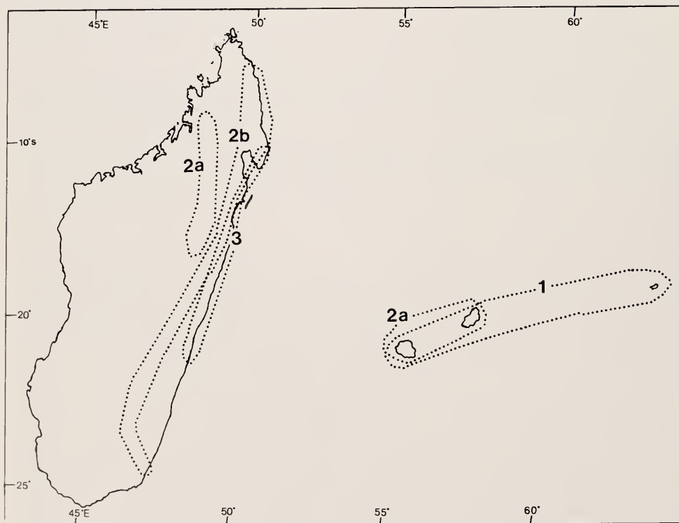
Map 1. Geographical distribution of Antirhea subgenus Antirhea . 1. A. bifurcata . 2a. A. borbonica var. borbonica . 2b. A. borbonica var. duplidentata . 3. A. madagascariensis .
